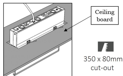
Cut-out for recessed version
